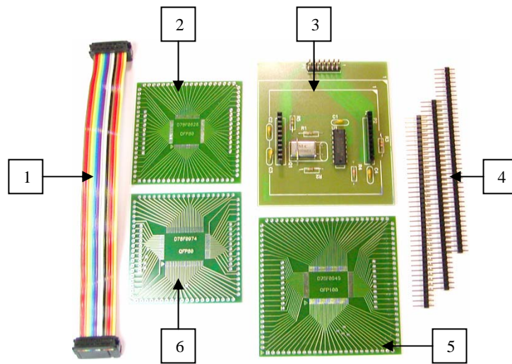
Figure 1 (adapters set)
